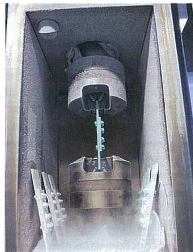
Phase II Mechanical & thermal preconditioning of sealant test vehicles
