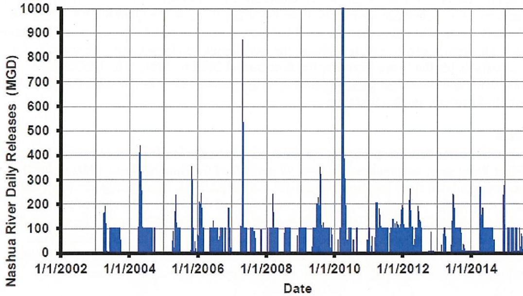
Figure 8 Nashua River Flow, MGD USGS Gage 01095503
