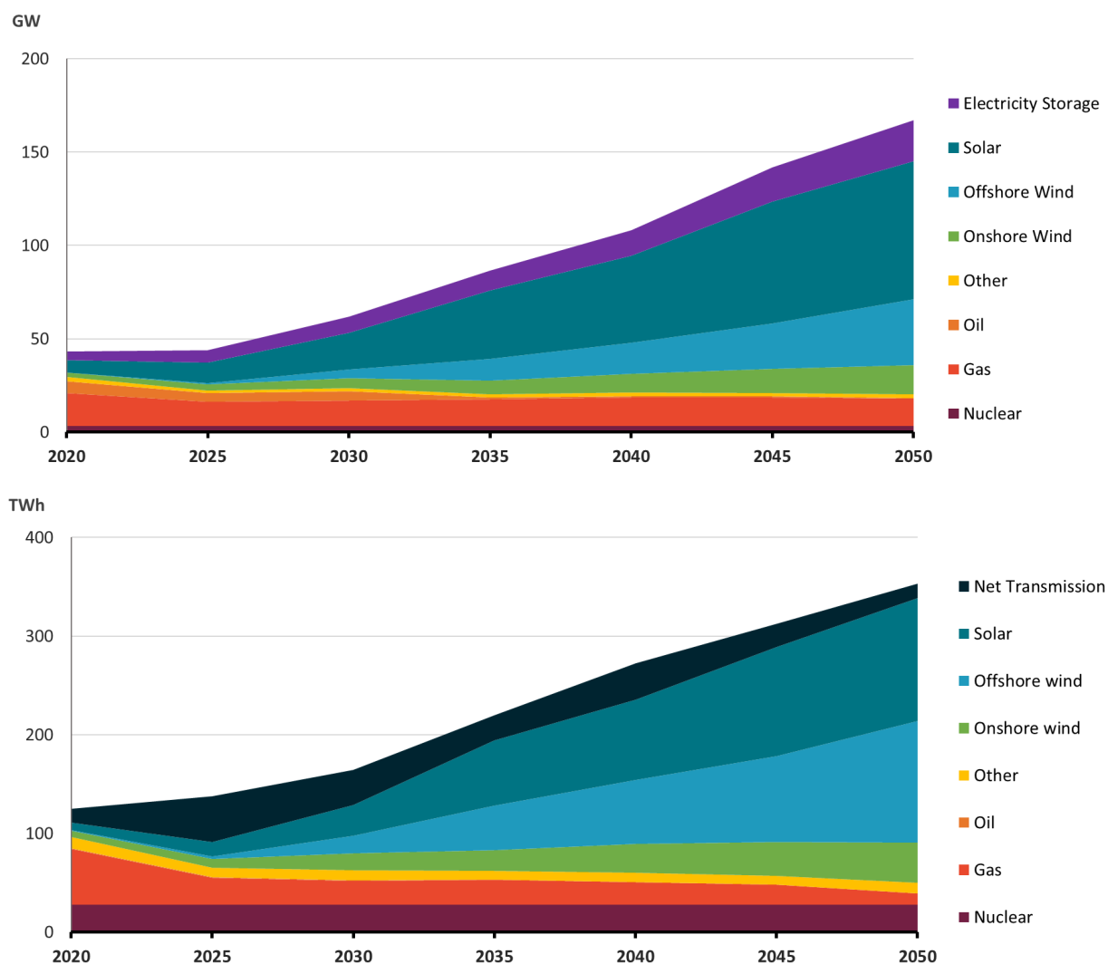
FIGURE 5C-1. NEW ENGLAND’S INSTALLED CAPACITY (TOP PANEL) AND ELECTRICITY GENERATION (BOTTOM PANEL) BY ENERGY SOURCE
