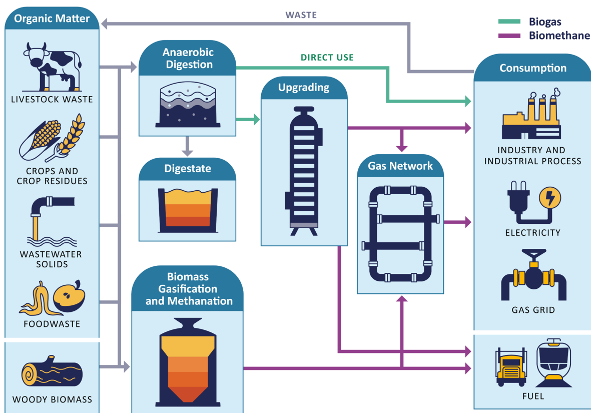
FIGURE 6-2. BIOGAS PATHWAYS 168
