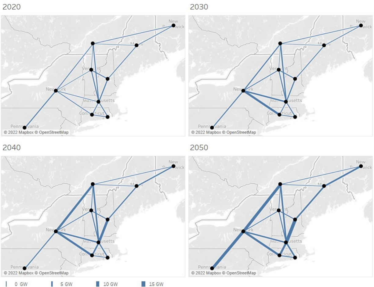
FIGURE 5C-2. ILLUSTRATIVE MAP OF TRANSMISSION CAPACITY NEEDED BETWEEN MASSACHUSETTS AND NEIGHBORING AREAS
