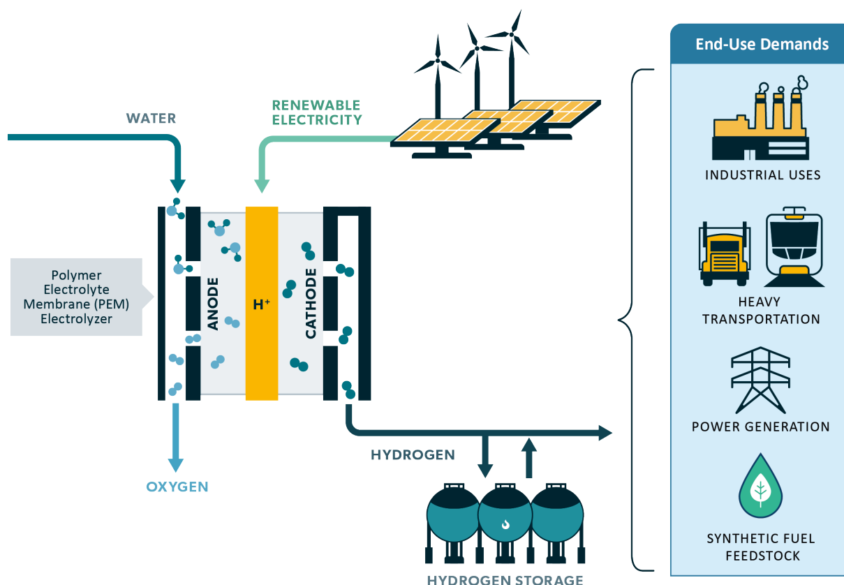
FIGURE 6-4. GREEN HYDROGEN PATHWAY
