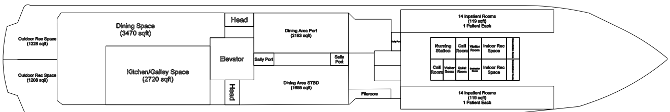
Figure 29: Deck 05
