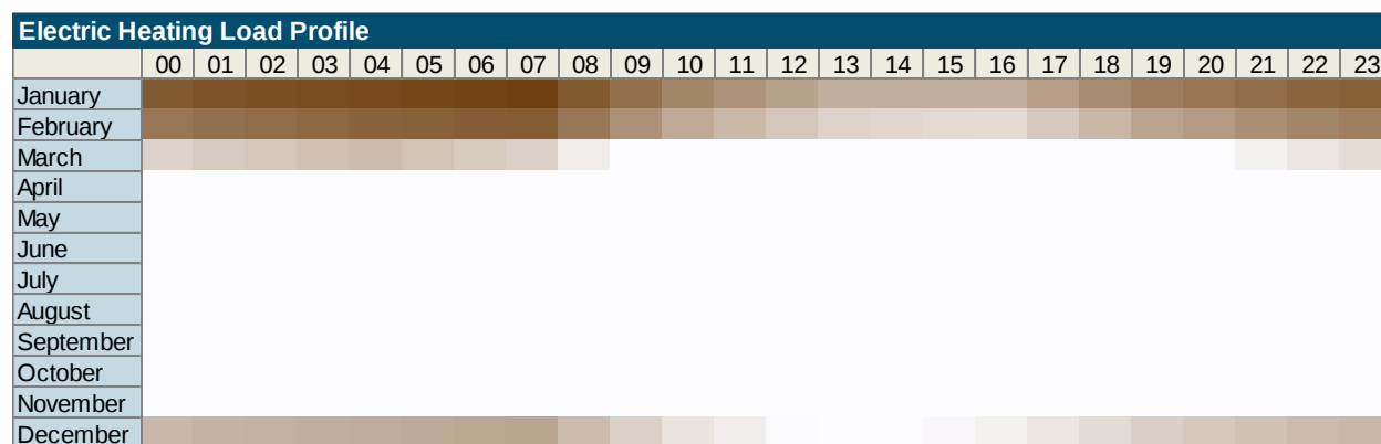
Figure 4-11. Month-Hour Average Electric Heating Loads, 2030
