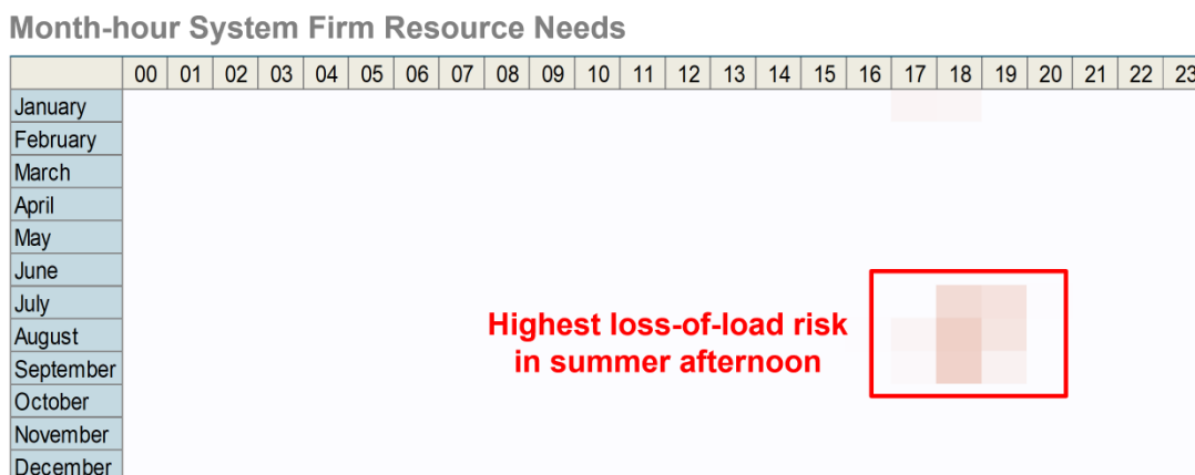
Figure 4-19. Average System Resource Need for ISONE under CECP Portfolio, 2030
