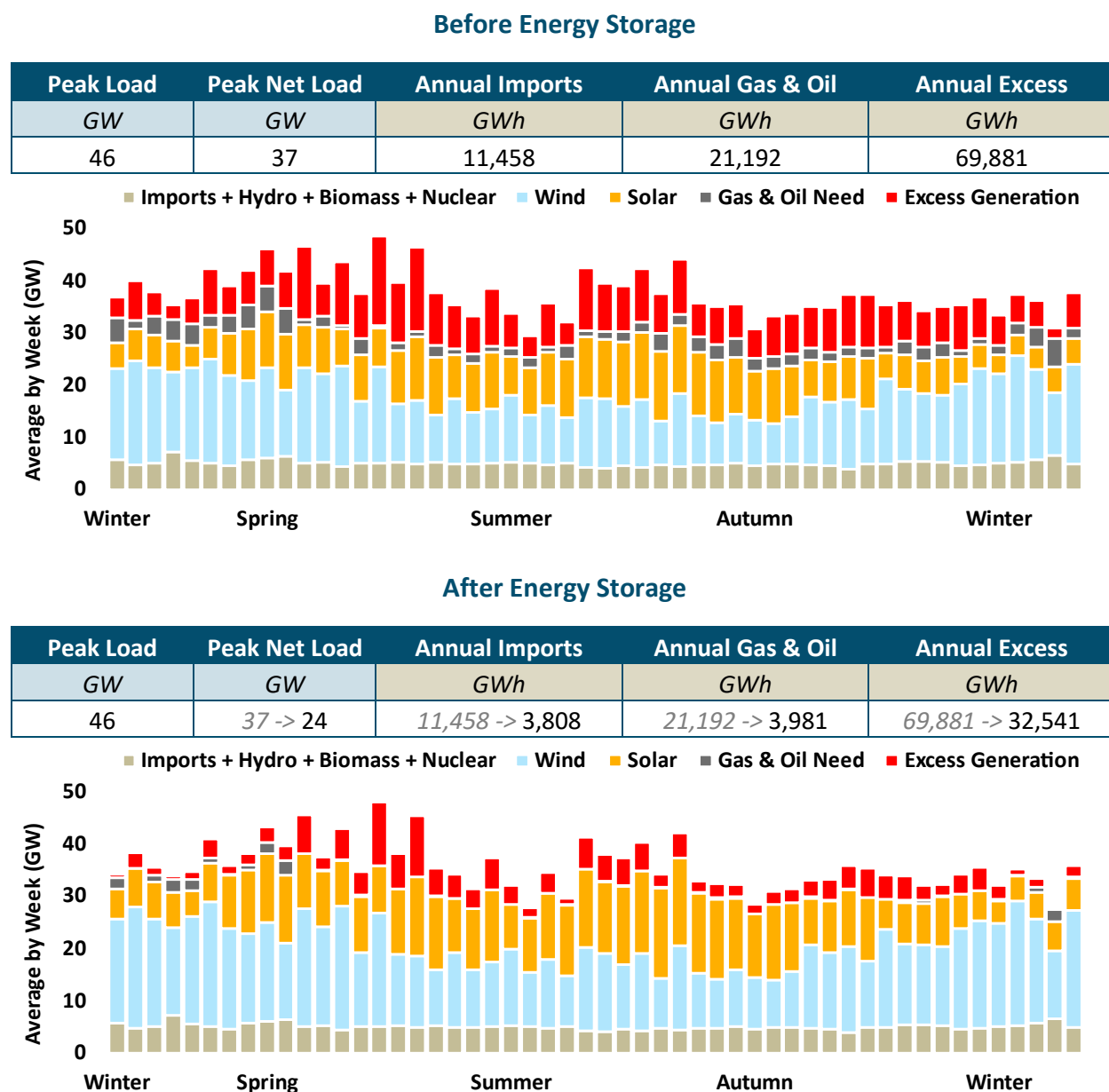
Figure 4-35. Example Simulated Low Peak and High Energy Excess Year
