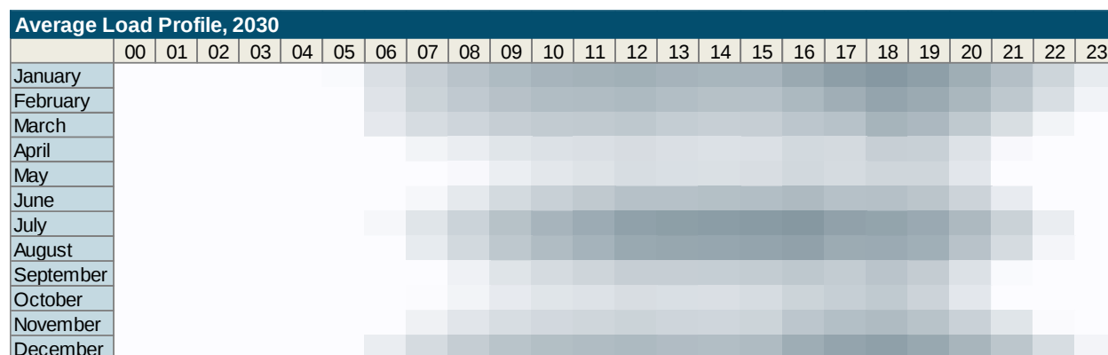
Figure 4-12. Month-Hour Average Total Loads in New England, 2030
