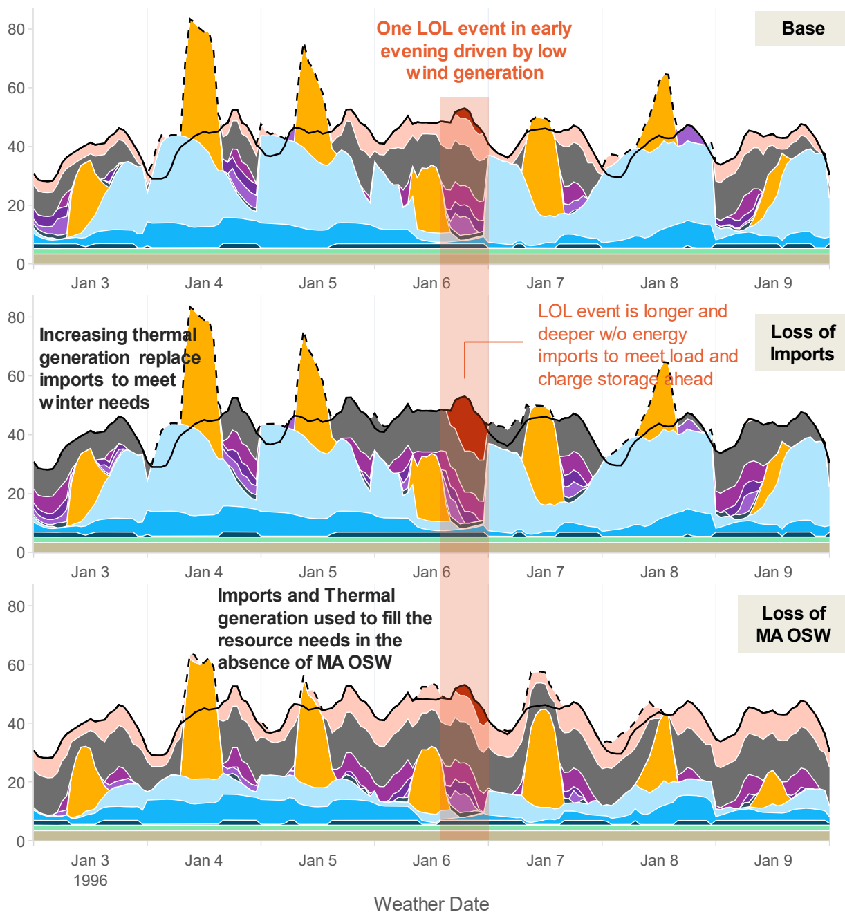
Figure E-5. Example winter week dispatch around loss-of-load event, 2050
