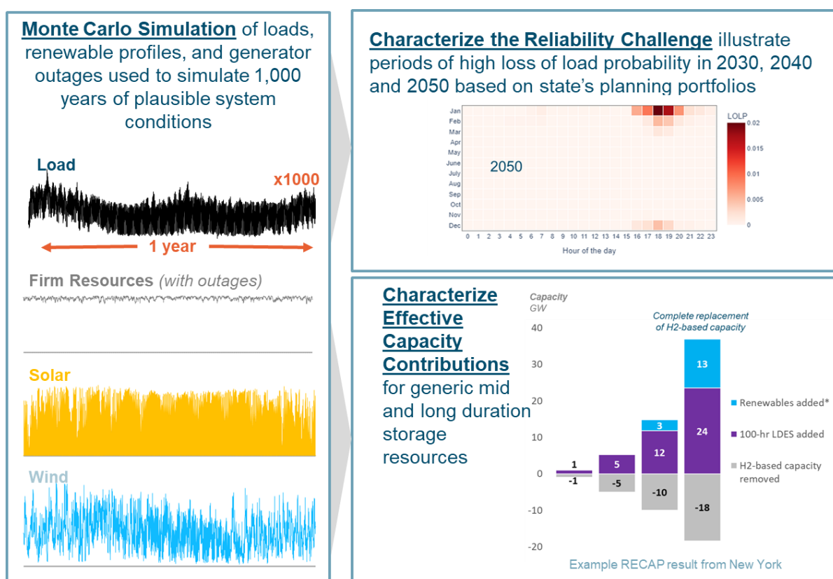
Figure 4-5. Overview of E3's RECAP Model
