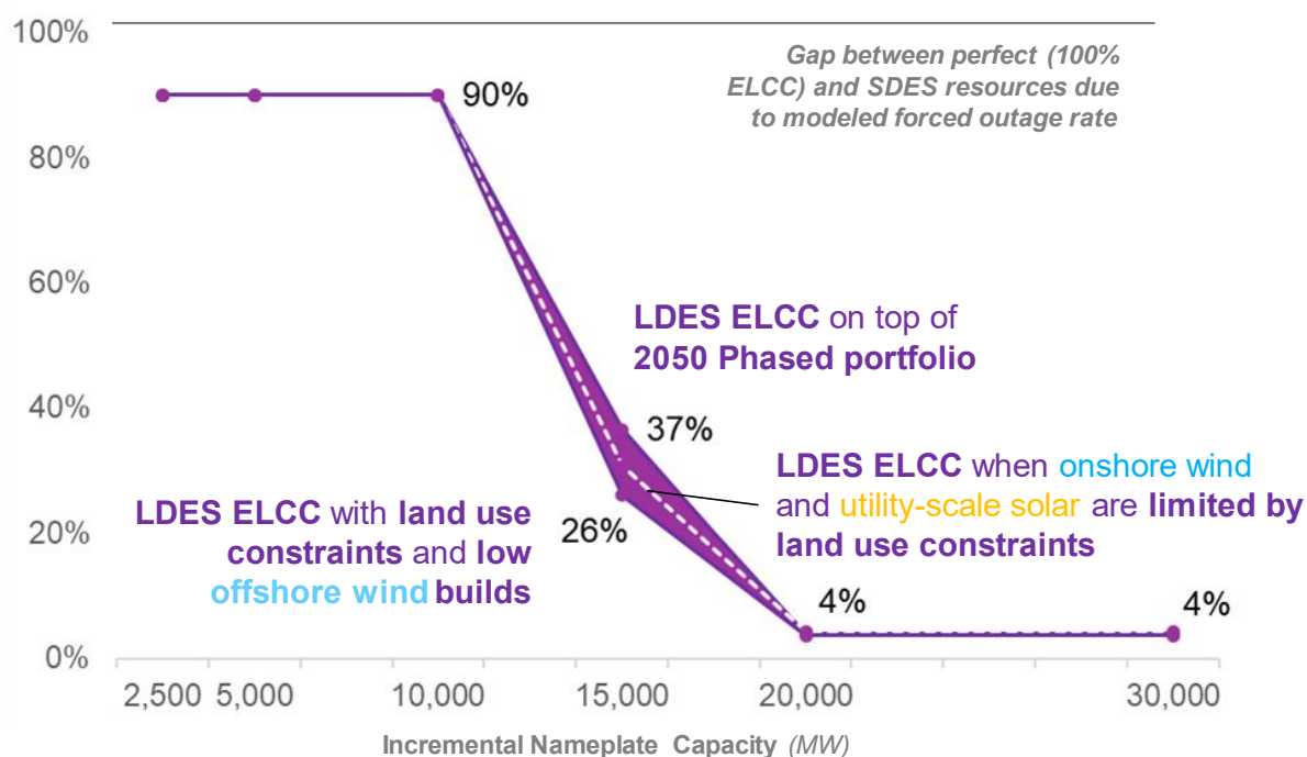
Figure 4-30. Incremental ELCC for Representative 100-hour Storage Resource, 2030
