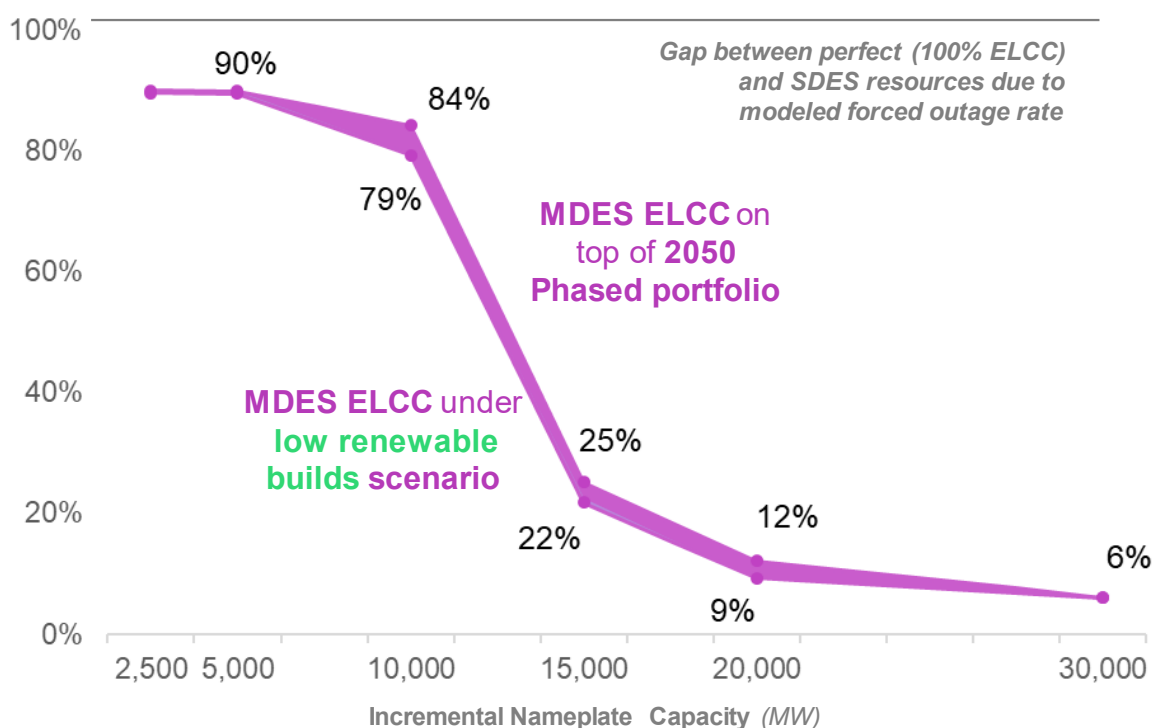
Figure 4-28. Incremental ELCC for Representative 8-hour Storage Resource, 2030
