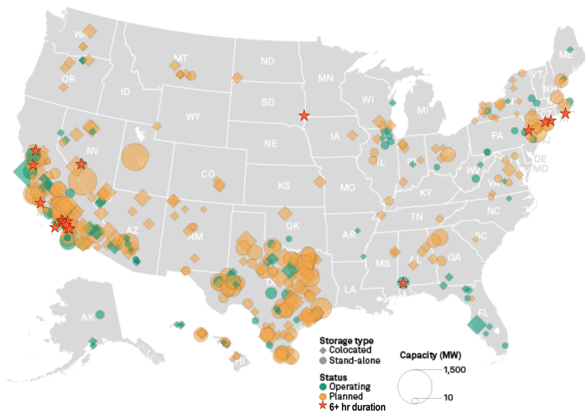
Figure 3-2. Utility-Scale Energy Storage Projects 46
