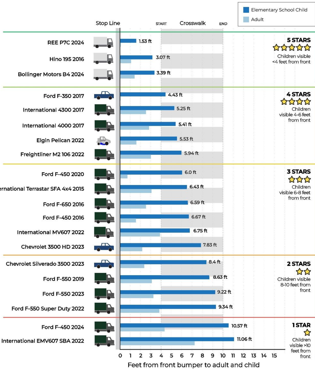
Figure 18. Nearest point at which an adult and child are visible to a driver at a standard crosswalk and stop bar overlaid with a five-star rating system for measured medium-duty vehicles.
