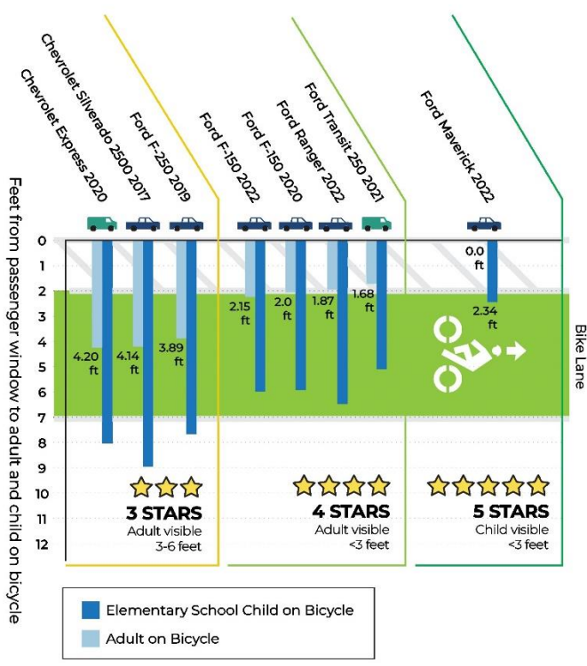
Figure 21. Nearest point at which an adult and child are visible to a driver at a buffered bike lane overlaid with a five-star rating system for measured medium-duty vehicles (top) and light-duty vehicles (bottom).
