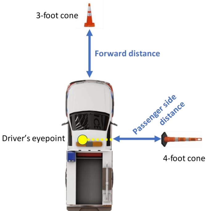
Figure 30. Proposed near-term cone method of direct vision reporting for bidders.
